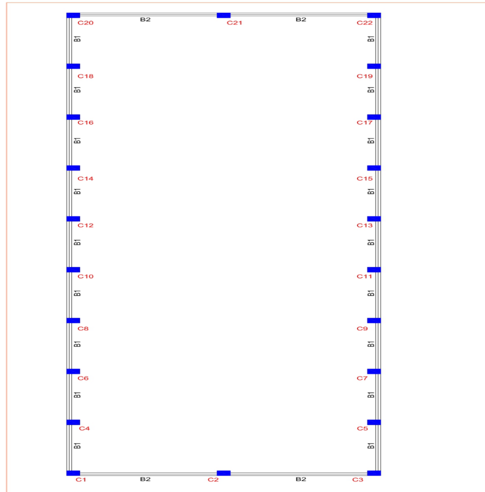
GROUND LEVEL RCC PLAN
