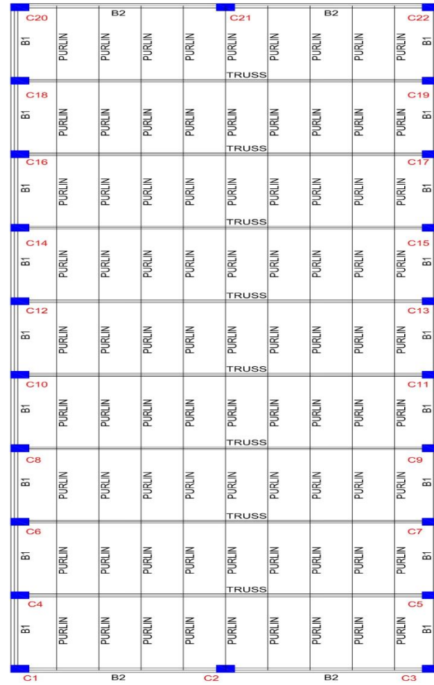
TRUSS BOTTOM PLAN
